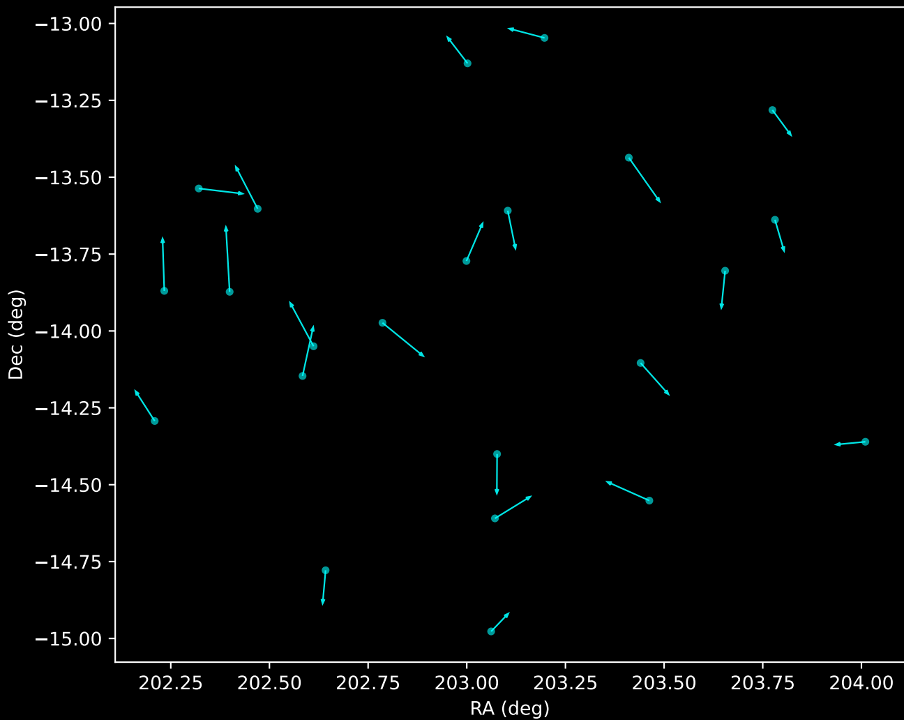
GALAH DR4 Noise Stream Proper Motion Vectors (n=23)
