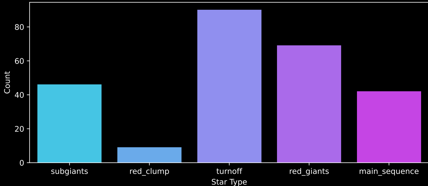
GALAH DR4 Field: [8754] Count plot of Star Type
