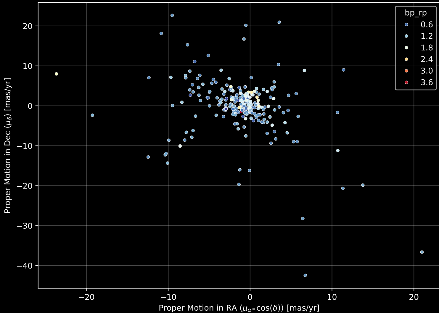
GALAH DR4 Field: [8754] Proper Motion Diagram (n= 256)
