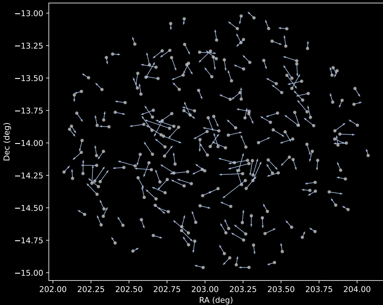
GALAH DR4 Cluster 1 Proper Motion Vectors (n=223)
