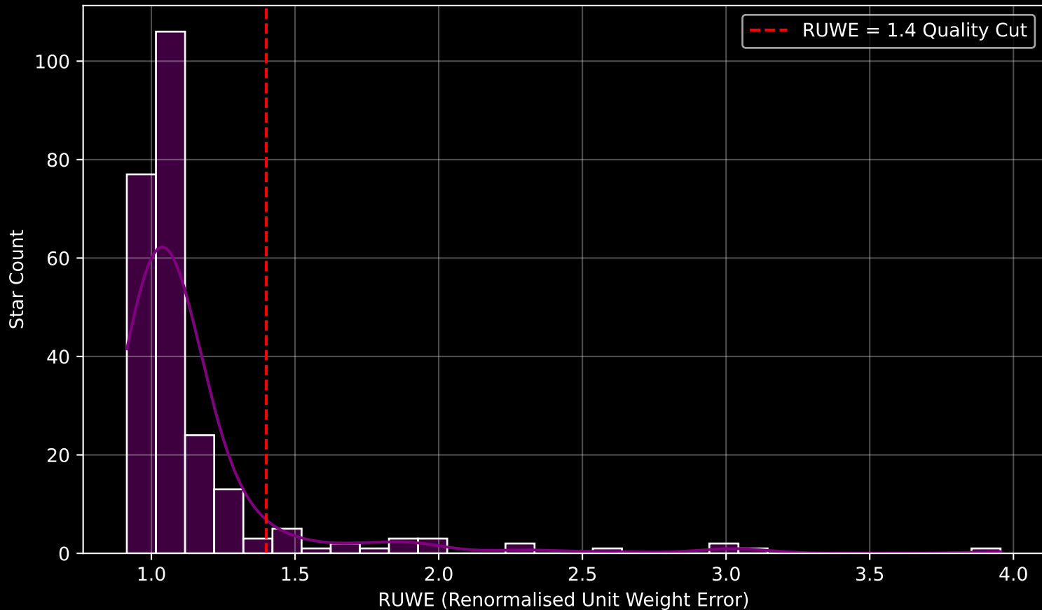
GALAH DR4 Field [8754] RUWE Distribution (n= 245)
